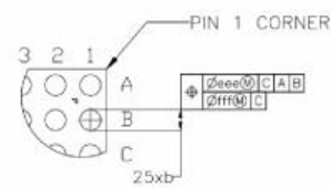
DETAIL A (2:1)
